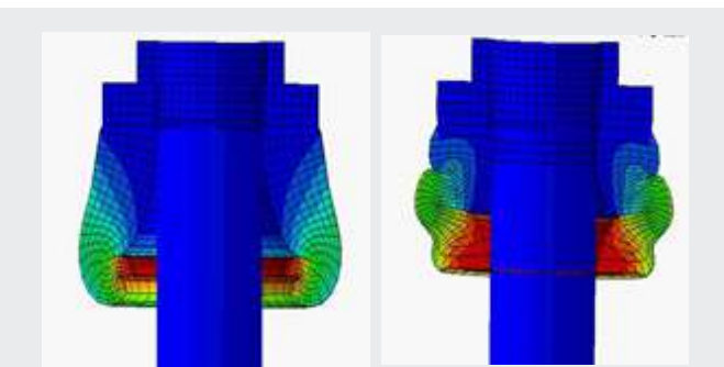
Fig. 4. Compressed behaviour of Initial (Left) and new (Right) design bump stop
